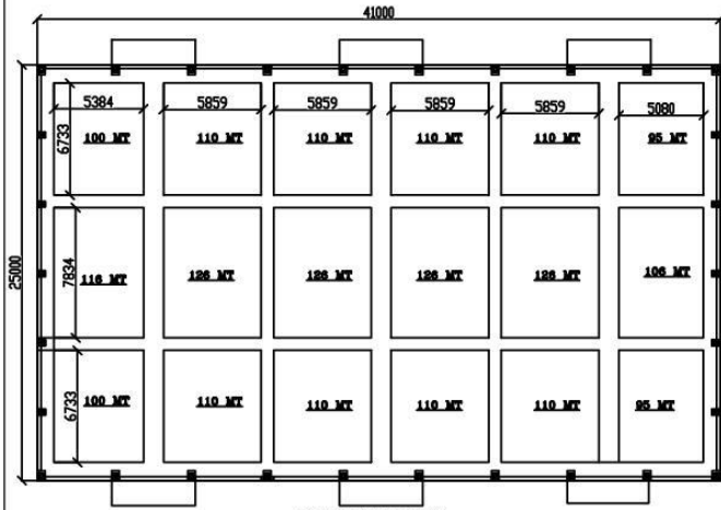
LAYOUT PLAN FOR 2000 MT WAREHOUSE
