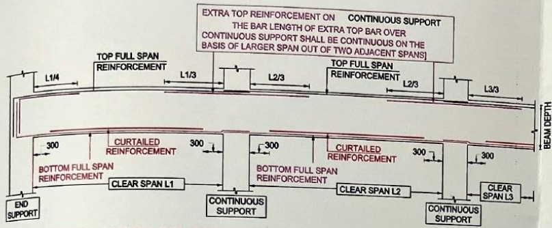
TYPICAL DETAILS FOR CURTAILMENT OF REINFORCEMENT FOR BEAMS.
