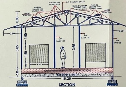
SECTION ONION STORAGE SHED
