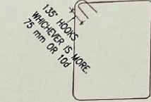
DETAIL OF BEAM STIRRUPS
