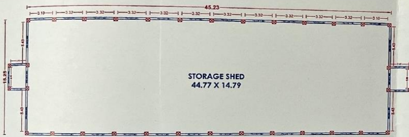
PLINTH BEAM LAYOUT PLAN ONION STORAGE SHED NO. 1 & 2
