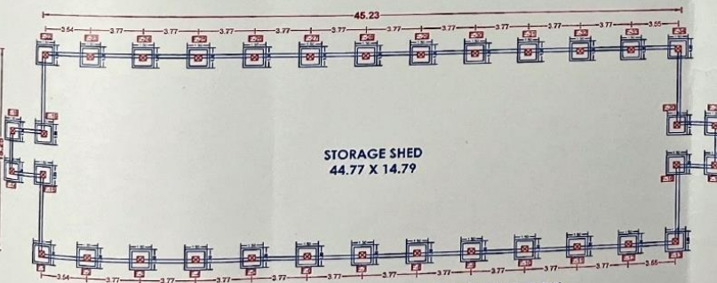
FOUNDATION LAYOUT PLAN & CENTERLINE PLAN ONION STORAGE SHED NO. 1 & 2
