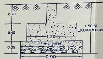
RCC FOOTING SECTION
