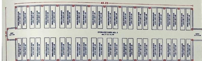
PLAN ONION STORAGE SHED NO. 2
