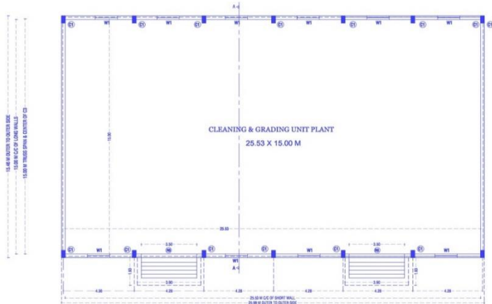
CLEANING & GRADING UNIT PLANT PLAN
