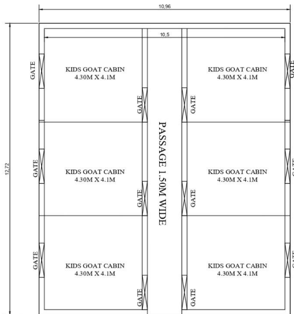
PLAN OF SHED FOR KID GOATS
