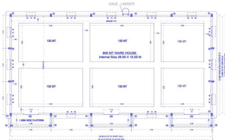
800 MT WARE HOUSE UNIT PLAN
