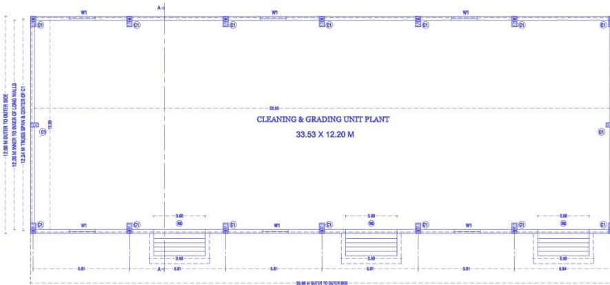
CLEANING & GRADING UNIT PLANT PLAN
