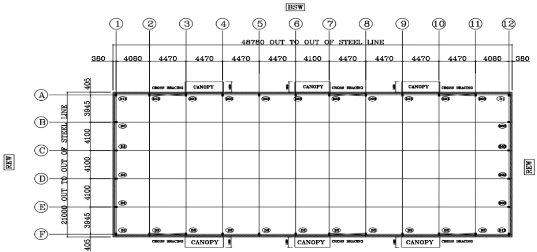
NSW ANCHOR BOLT PLAN FFL ±0.000M
