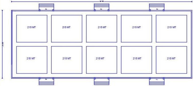
PLAN FOR 2150 MT WAREHOUSE SCALE 1:100
