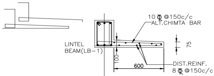
TYP. DETAILS OF CHAJJA
