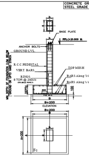
TYPICAL DETAILS OF FOUNDATIONS
