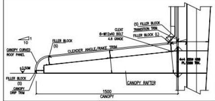
TYPICAL CANOPY DETAIL FOR SIDEWALL
