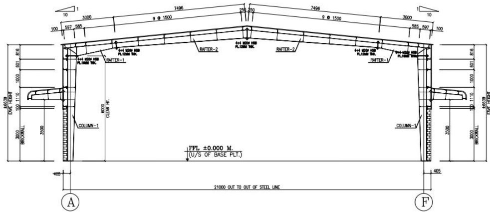
CROSS SECTION @ FRAME LINE 1 TO 12
